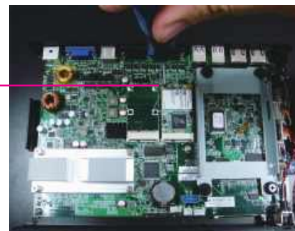
Mounting screw
